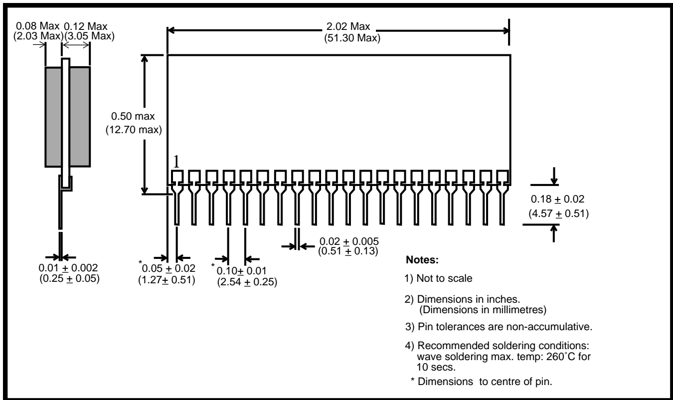
Figure 4 - Mechanical Data
